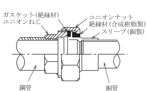
(7) 鋼管と銅管
